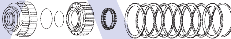
'C3' Clutch (3rd & 7th)
