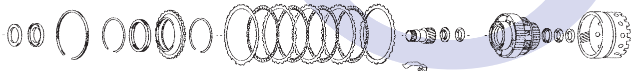
'F1' One Way Clutch, 'B2' Brake (Reverse) & Rear Planetary Assembly
