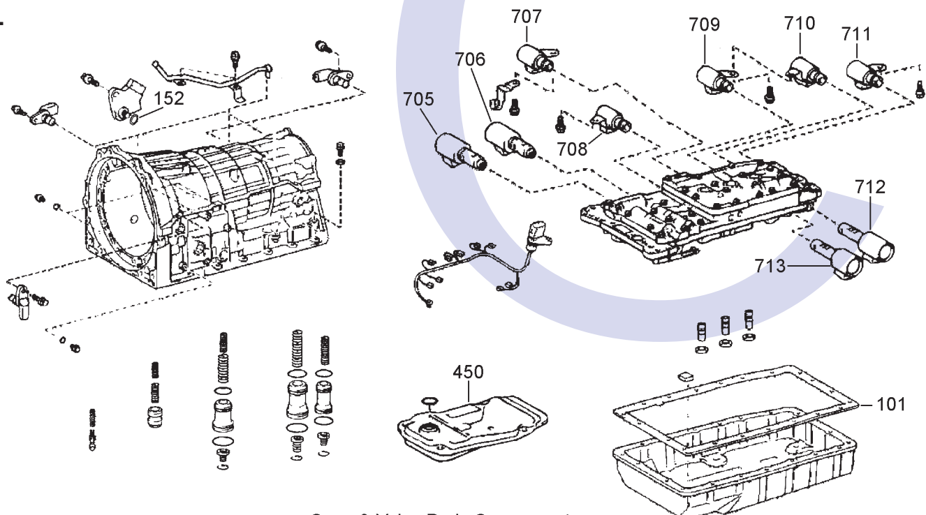
Case & Valve Body Components
